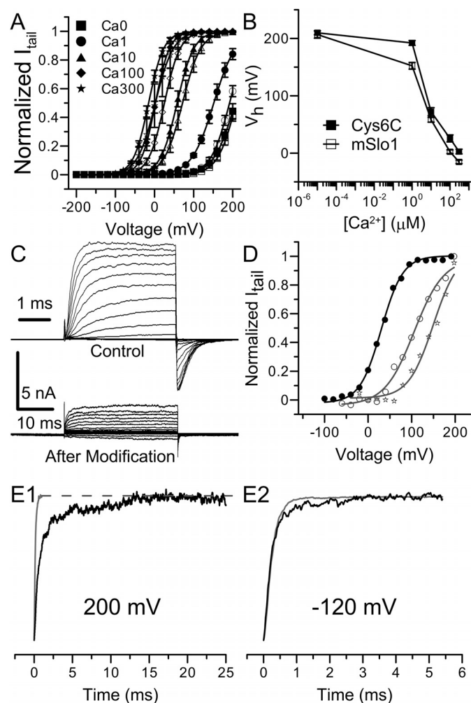
Fig. 8. Gating behavior and \text{Ag}^+ sensitivity of mSlo1Cys6C. A , The G-V curves of mSlo1Cys6C (filled symbols) in a wide range of [\text{Ca}^{2+}]_{\text{in}} overlap with those of mSlo1 (open symbols) in various [\text{Ca}^{2+}]_{\text{in}} : 0 \mu\text{M} (■), 1 \mu\text{M} (●), 10 \mu\text{M} (▲), 100 \mu\text{M} (◆), and 300 \mu\text{M} (★). Each set of data is averaged from five patches. Lines are Boltzmann fits. B , the V_h values of mSlo1Cys6C and BK channels are plotted against [\text{Ca}^{2+}]_{\text{in}} (in log scale). The connecting lines have no physical meaning. C , macroscopic mSlo1Cys6C currents recorded in 100 \mu\text{M} [\text{Ca}^{2+}]_{\text{in}} before (top) and after (bottom) 240-s perfusion in 520 \text{ nM} \text{Ag}^+ . The voltage protocol was similar to the one used in Fig. 2A. Notice that the time scales are different in these two sets of recordings. D , the macroscopic G-V profiles of mSlo1Cys6C in 100 \mu\text{M} \text{Ca}^{2+} before \text{Ag}^+ modification (●), and in 10 \mu\text{M} \text{Ca}^{2+} after \text{Ag}^+ modification (○). The Boltzmann fitting results were as follows: V_h = 30 \text{ mV} , z = 1.02 ( 100 \mu\text{M} \text{Ca}^{2+} before \text{Ag}^+ treatment); V_h = 150 \text{ mV} , z = 0.88 ( 10 \mu\text{M} \text{Ca}^{2+} after \text{Ag}^+ treatment); V_h = 106 \text{ mV} , z = 0.74 ( 100 \mu\text{M} \text{Ca}^{2+} after \text{Ag}^+ treatment). E , normalized activation (E1, 200 \text{ mV} ) and deactivation (E2, -120 \text{ mV} ) time course of mSlo1Cys6C currents before (gray) and after (black) \text{Ag}^+ modification.
