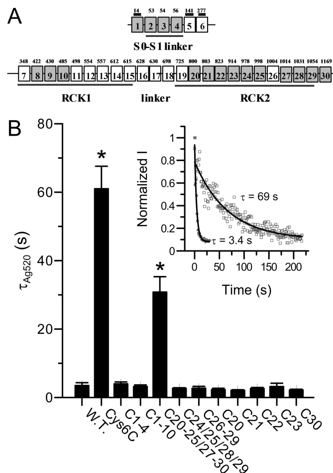
Fig. 7. Ag + sensitivity of various cysteine-less constructs. A, the schema maps the linear distribution of 30 cysteines on the BK channel. Top row, cysteines on the extracellular side and in the transmembrane segments of BK channel. Bottom row, the cysteines in the cytosolic domain. Three extracellular cysteines are marked by bars above squares. The number in each square refers to the sequential number of that cysteine. The numbers above squares are the actual positions of cysteines in mSlo1. In mSlo1Cys6C, 17 of these cysteines are mutated into serines (shaded). B, the mean modification time constants of various cysteine-less constructs by 520 nM Ag + : wild type ( 3.5 \pm 0.8 s, n = 6 ), Cys6C ( 61 \pm 6.6 s, n = 9 ), Cys1 to Cys4 ( 3.9 \pm 0.6 s, n = 5 ), Cys1 to Cys10 ( 3.2 \pm 0.45 s, n = 6 ), Cys20–25/27–30 ( 30.8 \pm 4.5 s, n = 8 ), Cys24/25/28/29 ( 2.7 \pm 0.2 s, n = 6 ), Cys26 to Cys29 ( 2.7 \pm 0.5 s, n = 4 ), Cys20 ( 2.3 \pm 0.4 s, n = 5 ), Cys21 ( 2.1 \pm 0.2 s, n = 4 ), Cys22 ( 2.64 \pm 0.28 s, n = 5 ), Cys23 ( 3.2 \pm 0.97 s, n = 4 ), and Cys30 ( 2.2 \pm 0.3 s, n = 4 ). Only Cys6C and Cys20–25/27–30 show significantly reduced Ag + sensitivity, as marked by asterisks. Inset, the time course of modification on mSlo1Cys6C (□) by 520 nM Ag + overlapped with that of wild type BK (●) at the beginning of Ag + application, as indicated by time 0.
